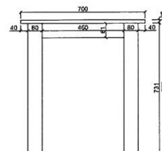
bokorys M 1:20
