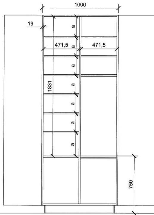
bokorys M 1:20
